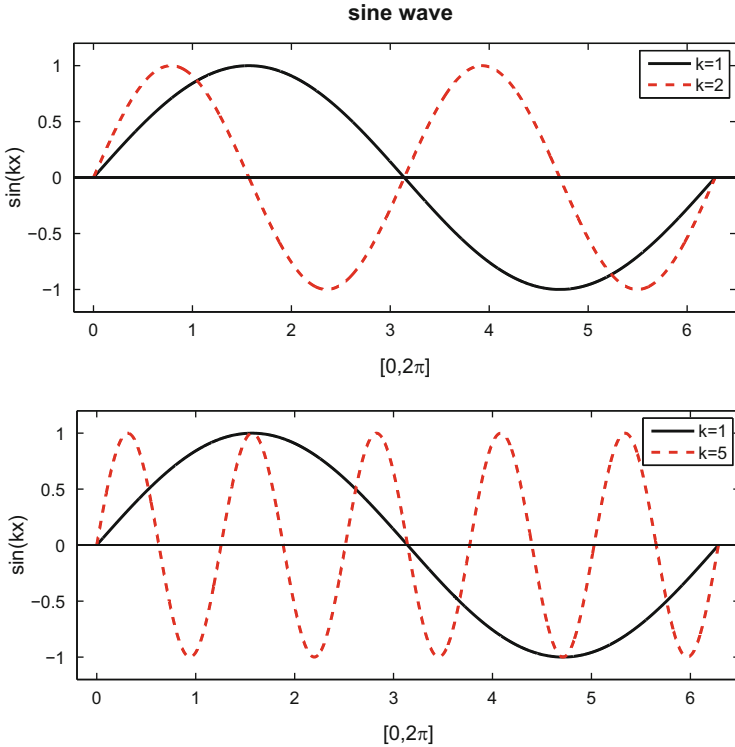
Fig. 10.1 Sine cycles of different frequencies (Example 10.5)
