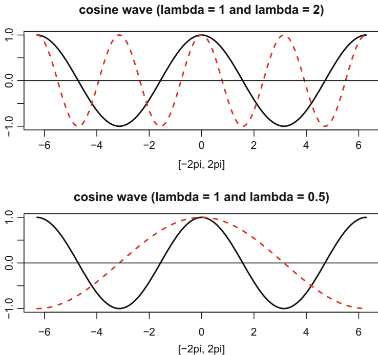
Fig. 4.1 Cosine cycle with different frequencies
