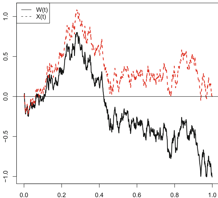
Fig. 7.5 WP and Brownian bridge ( \sigma = 1 )
